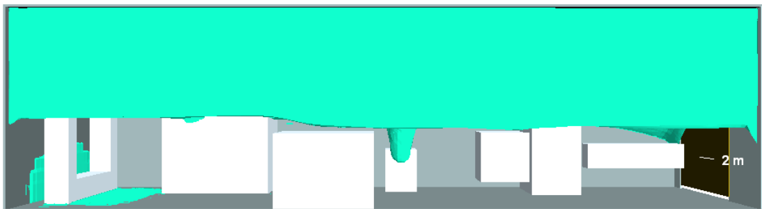
Figure 10 Zone with temperatures above 20°C (no fans)
