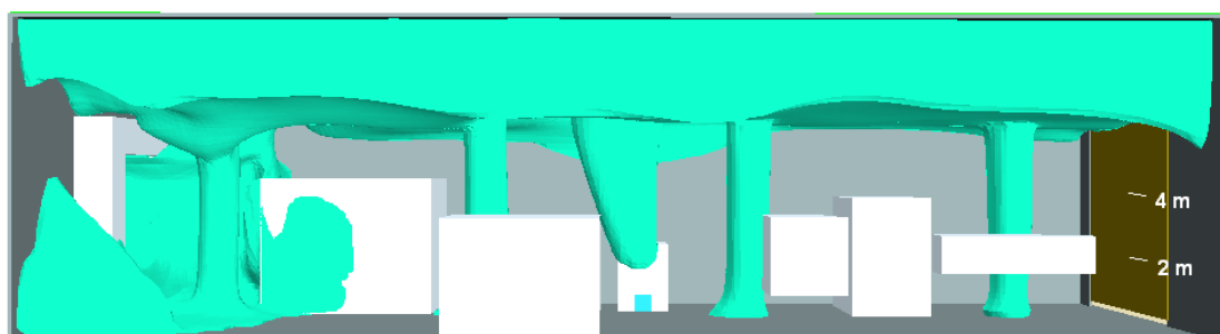
Figure 12 Zone with temperatures above 20°C (with four fans)
